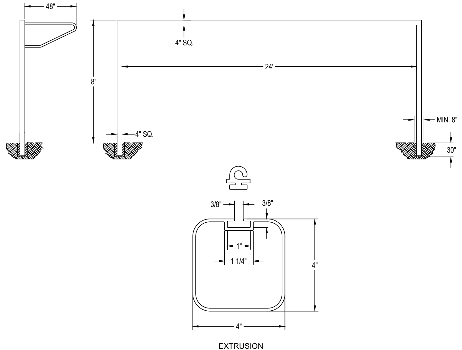
EXTRUSION
