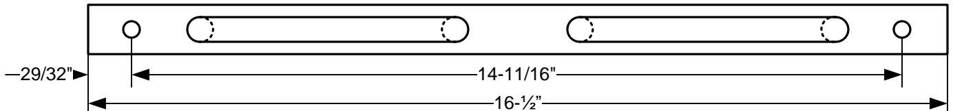
BOTTOM BRACKET
