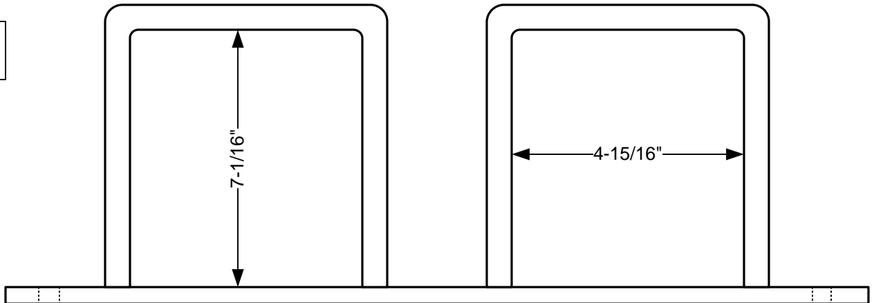
BOTTOM BRACKET
