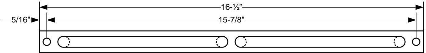
TOP BRACKET
