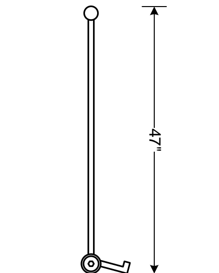
TRANSPORT DOLLY
